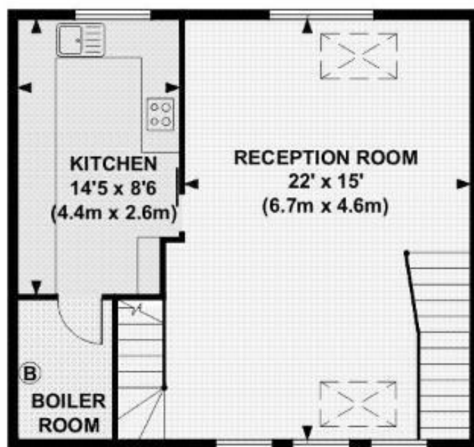
FIRST FLOOR GROSS INTERNAL FLOOR AREA 522 SQ FT
